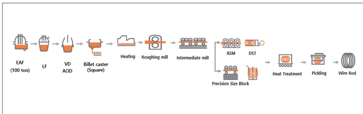
Figure 2 Manufacturing Process
